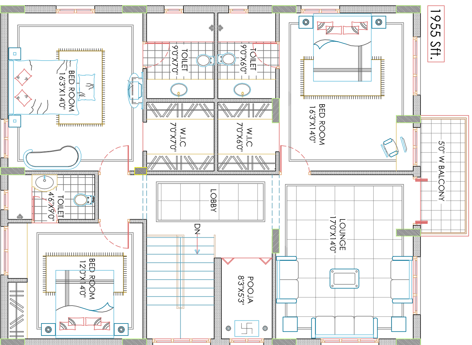
SECOND LEVEL PLAN
