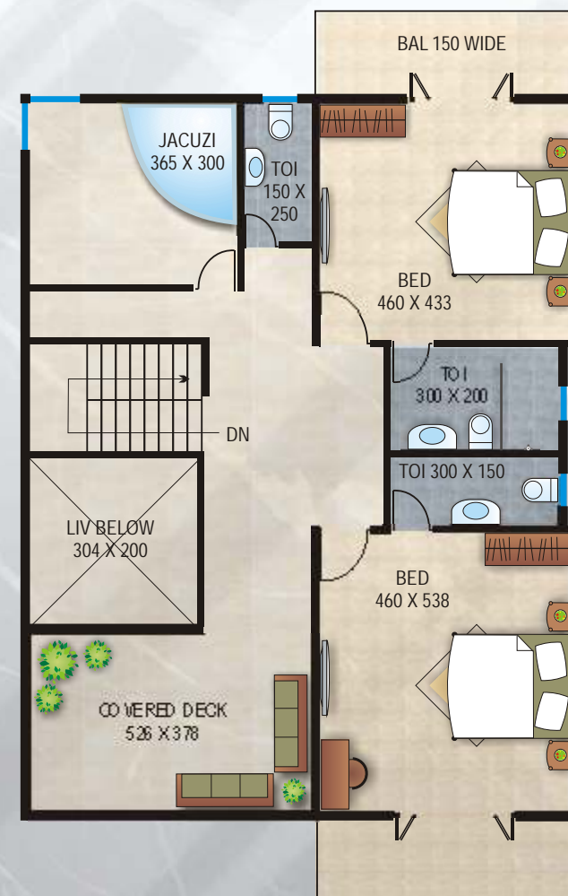
FIRST FLOOR PLAN - B
