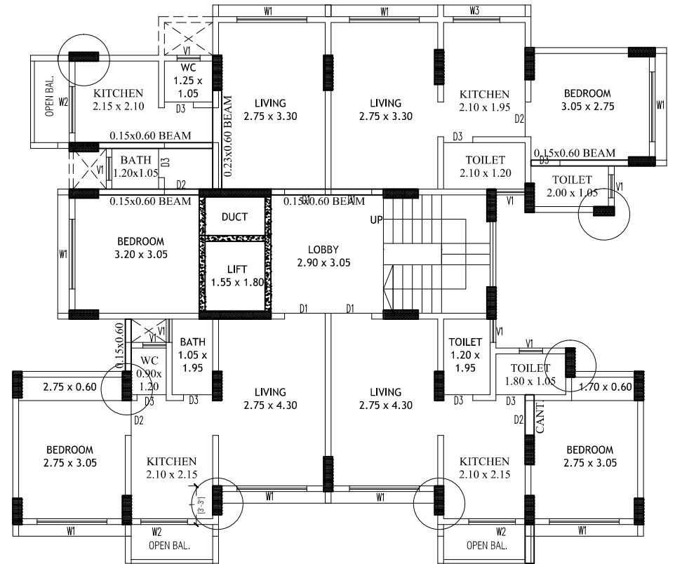
TYPICAL FLOOR PLAN (1ST, TO 7TH FLOOR) (BUILDING NO.4) TYPE A SCALE: 100
