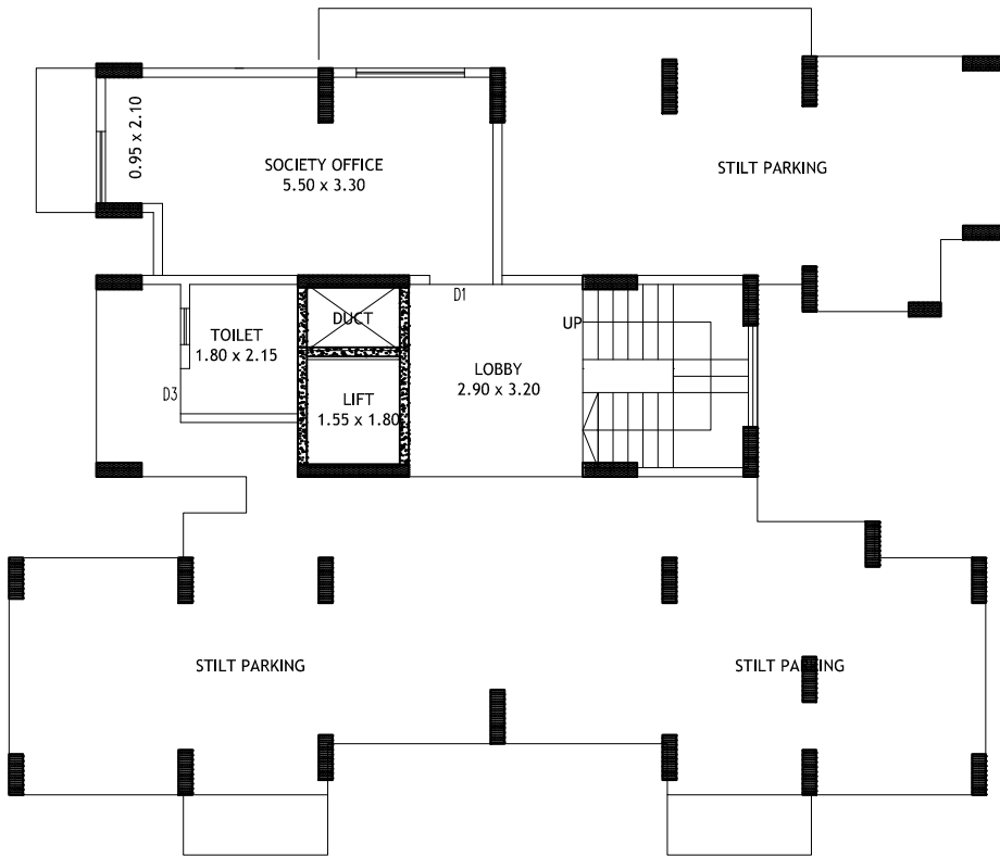
GROUND FLOOR PLAN (BUILDING NO.4) TYPE A SCALE 1 : 100
