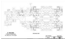
1 & 2 BHK Typical
