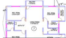
Floor Plan-D
